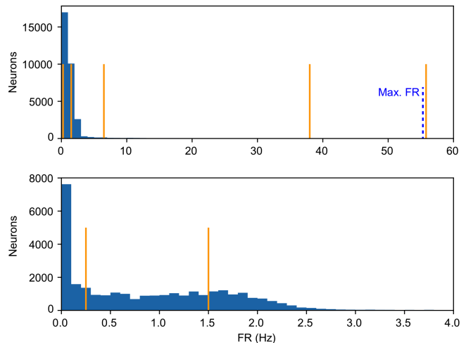
Figure 10: Distribution of neuron counts by spiking rates collected from the central minicolumn (31346 neurons) of the network utilized in the simulation of the laboratory experiment described in Section 3.4, in the interval 2-4 secs. Orange bars represent the frequencies 0.25 Hz, 1.5 Hz, 6.5 Hz, 38 Hz and 55 Hz that describe the boundaries of the 5 spiking regimes analysed. Top: a bin accounts for 1Hz. Max. FR is the maximum firing rate measured; Bottom: zoomed dataset with a cut off at 0-40 Hz. A bin accounts for 0.1 Hz.
