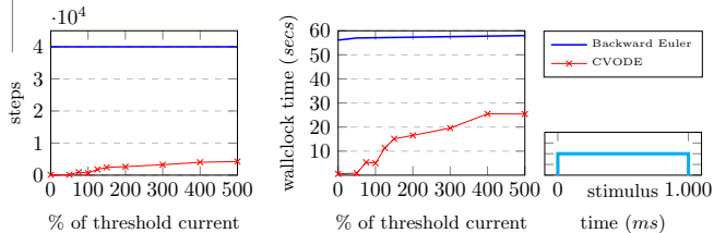
Figure 6: Interpolation steps and runtime for the 1000ms simulation of the injection of a continuous current as a percentage of the threshold current ( 0.206mA ) on a layer 5 pyramidal cell (L5_TTPC2_cADpyr232_1 [16]). Results presented for the Backward Euler with \Delta t = 25\mu s and CVODE with atol=10^{-3} . Hardware specs.: Intel core i5 at 1.6 GHz.
