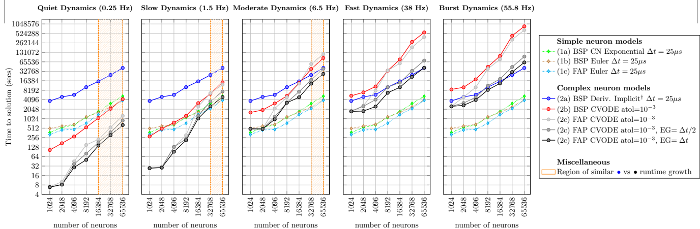
Figure 9: Runtime for the simulation of one second of biological activity of neuron networks described by five spiking rate dynamics. Results measured for increasing input sizes on a network of 64 Cray XE6 nodes, with an AMD Opteron 6380 with 16 cores at 2.5 GHz. Key: BSP: Bulk Synchronous Parallel; FAP: Fully-Asynchronous Parallel; atol: absolute tolerance; EG: event grouping interval; †: able to solve non-linear ODEs implicitly, and unable to solve correlated mechanism states implicitly.
